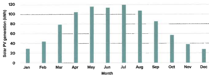
Figure 6 – Typical monthly solar PV generation (in kWh) for a typical 1 kW PV system in Wakefield
